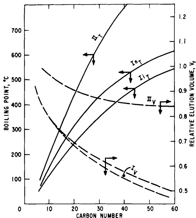
FIG. 1. Correlation of boiling point, relative elution volume, and carbon number for petroleum compounds. (—) Boiling point; (---) GPC (Poragel/methylene chloride). Ii = branched paraffins; In = n -paraffins; II = condensed rings.
